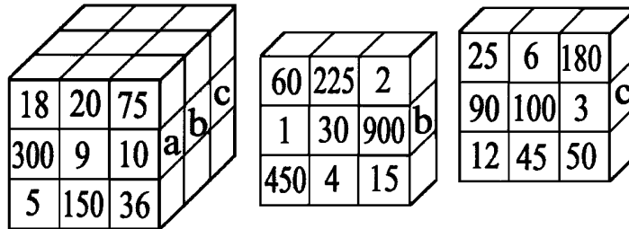
Fig. 2. Multiplicative magic cube \mathbf{Q}_3
